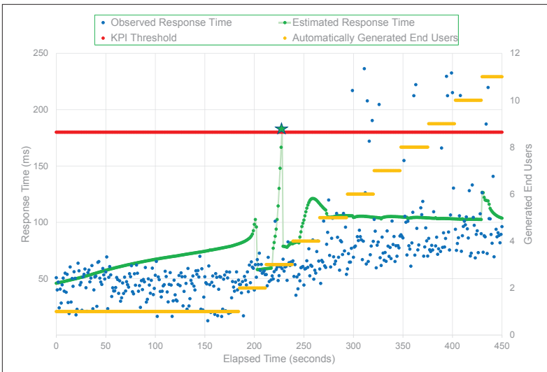
FIGURE 3. Estimated response time vs. observed response time as a function of the number of Cassandra users.
